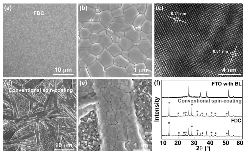
Figure 2. Morphological and structural characterization of \text{CH}_3\text{NH}_3\text{PbI}_3 films prepared by FDC and a conventional spin-coating process. The concentration of the perovskite solution was 45 wt %. a,b) Low- and high-magnification SEM images of the surface of a \text{CH}_3\text{NH}_3\text{PbI}_3 film prepared by FDC with the addition of chlorobenzene. c) An atomic resolution TEM image of a \text{CH}_3\text{NH}_3\text{PbI}_3 grain from a film produced by FDC, showing a pseudo-cubic lattice. d,e) Low- and high-magnification SEM images of a film prepared by conventional spin-coating. f) XRD patterns of the films corresponding to (a) and (d). The XRD pattern of the \text{TiO}_2 blocking layer (BL) coated FTO substrate is shown for comparison. The XRD peak intensity has been normalized. The peaks assigned to \text{CH}_3\text{NH}_3\text{PbI}_3 crystals are marked with asterisks.
